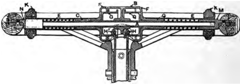
FIG. 234.—Steering Wheel and Attachments of the Panhard-Levassor Carriage. A, a shaft on a diameter of the wheel; B, a cylindrical fixed cap with toothed end; C, C, a sleeve with toothed ends, F, F, in normal engagement with B, under tension of springs, E, E, being prevented from rotating; G, G, drums on which wire cables, H, H, are secured and wound; K, K, knurled handles which may be grasped and pulled against the springs, allowing rotation of G, G. One cable, H, leads to carburetter link, the other to the spark adjuster.
